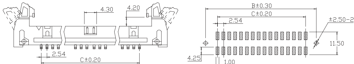
Recommended PCB Layout (PCB TOLERANCE±0.05)
